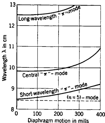
FIG. 14-20.—Tuning curves of 4J75 magnetron.
